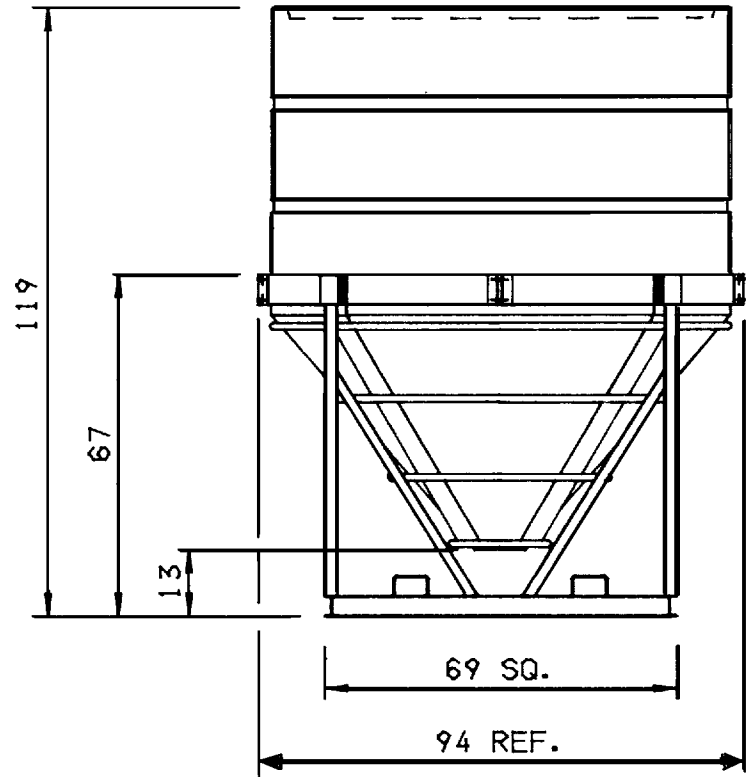
TANK WITH STAND & BASKET
